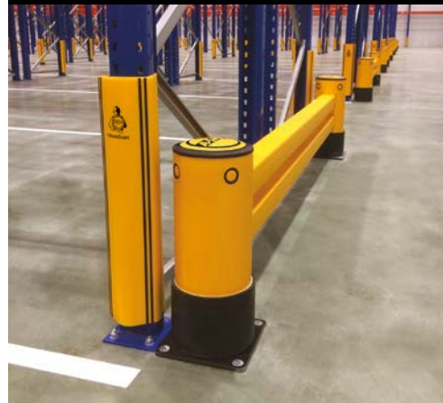
eFlex Single Rackend Barrier
